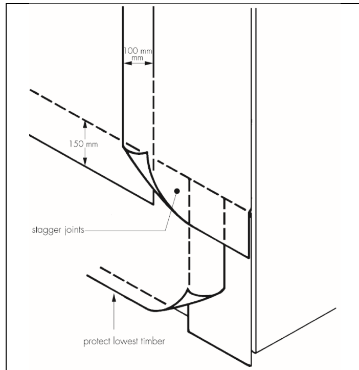
Figure 1 Membrane installation
