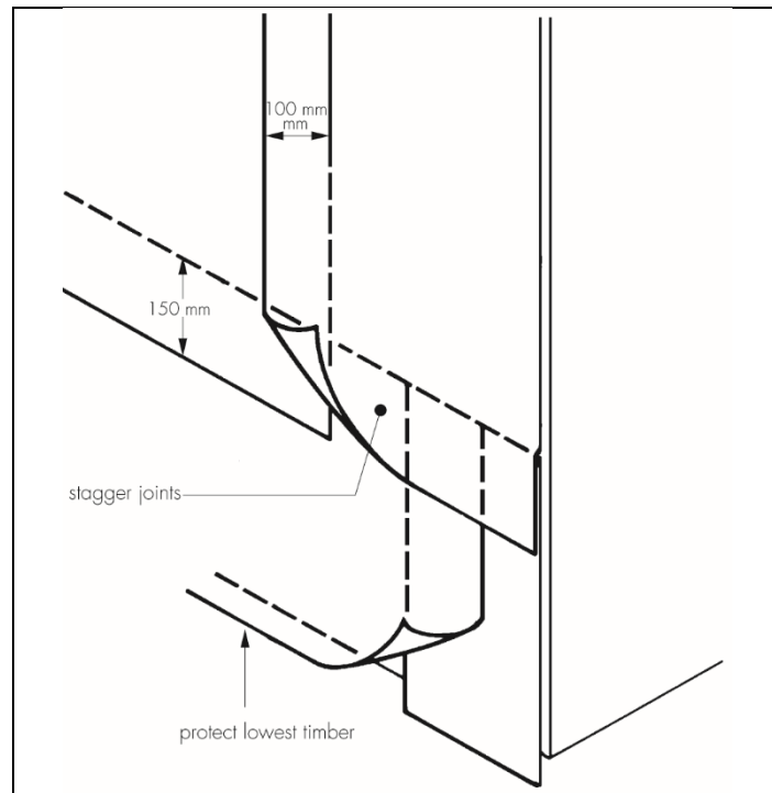
Figure 1 Membrane installation
